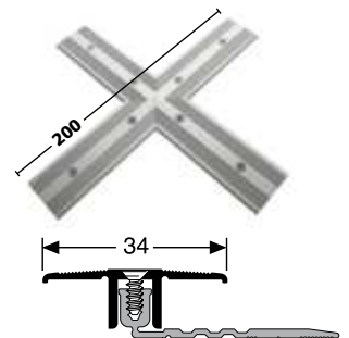
PF 488 FK \varnothing 7-15 mm 360° Fugenkreuz 360° Crossing joint 360° Croix
