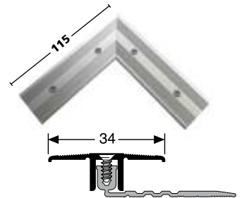
PF 488 EC \varnothing 7-15 mm 90° Ecke 90° Corner 90° Angle
